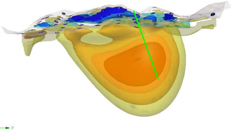
Image 1. Taguas MT survey, 3D inversion model resistivity iso-surfaces (shells) around low resistivities (10, 20, 50, and 100 \Omega\text{m} in red, orange, beige and yellow respectively) and high resistivities above 3,800 masI and west of 2415800mE (300 and 500 \Omega\text{m} , light and dark blue respectively) viewed sideways on from the east. Green line represents planned drillhole TADD278
