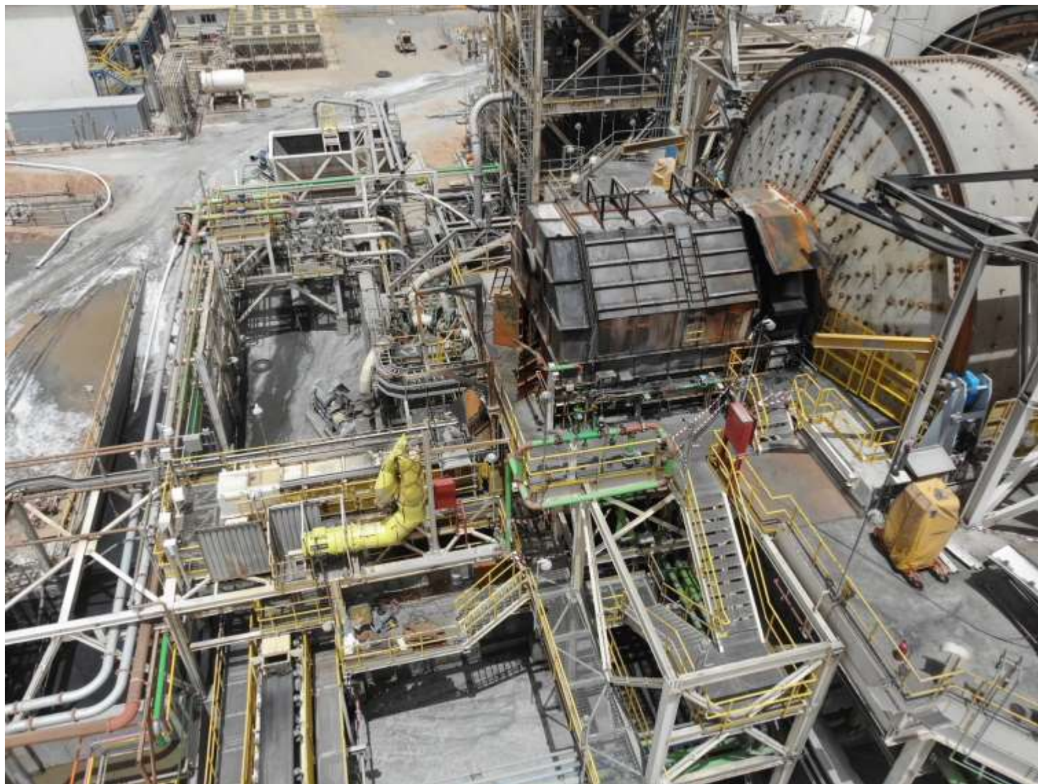
Figure 2: SAG mill discharge end with trommel screen
