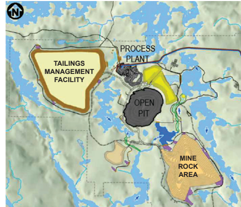
Site layout of the Côte Gold Project.
